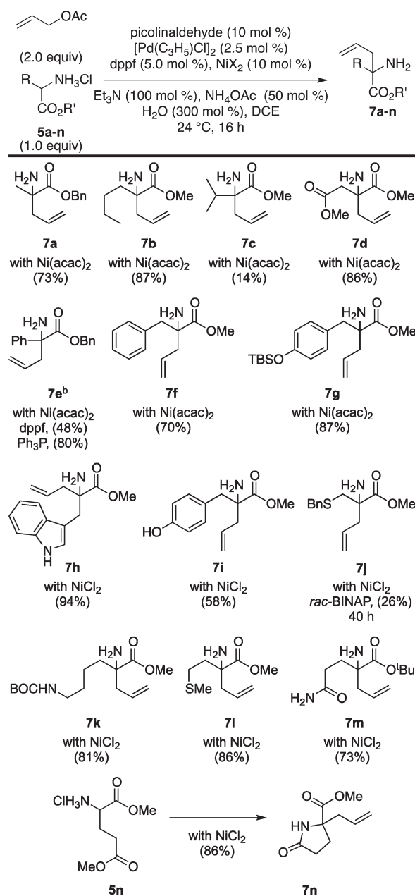
Figure 2. Reaction scope. a Yields given are isolated yields. b Reaction run using the tosylate salt of phenylglycine methyl ester.
