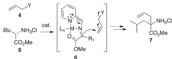
Scheme 1. Picolinaldehyde-Catalyzed Amino Acid Allylation
