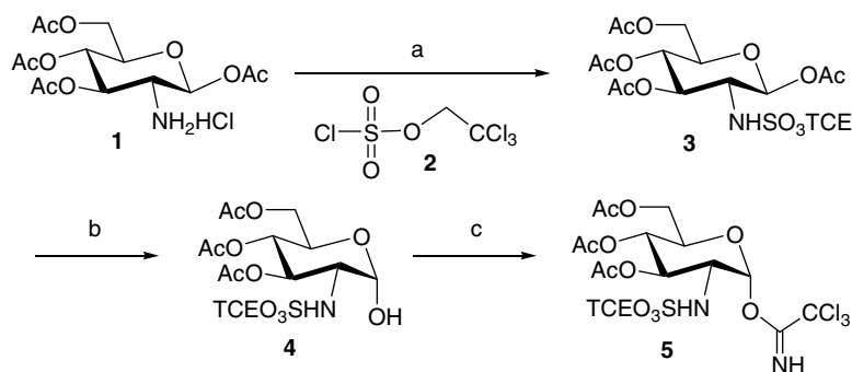
Scheme 1. Reagents and conditions: (a) \text{Et}_3\text{N} (3.5 equiv), DMAP (1 equiv), DMF, 0^\circ\text{C} , 2 h, 82%; (b) \text{NH}_3 , THF/MeOH (7:3), 0^\circ\text{C} , 15 min, 81%; (c) \text{CNCCl}_3 (3.0 equiv), \text{K}_2\text{CO}_3 (1.2 equiv), \text{CH}_2\text{Cl}_2 , rt, 10 h, 88%.
