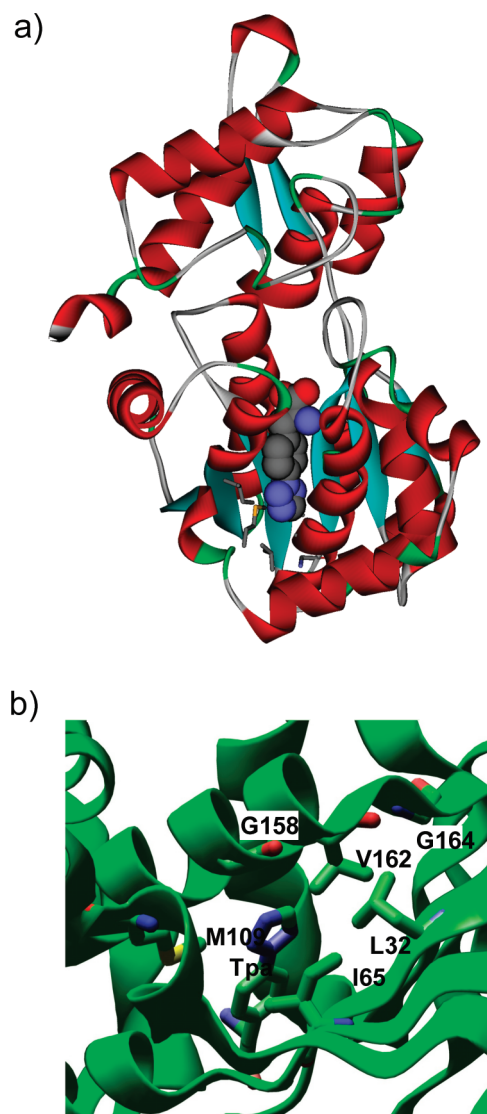
Figure 5. Crystal structure of p -TpaRS-1 bound to p -Tpa: (a) A ribbon model showing the overall fold with the bound p -Tpa ligand in the CPK model. (b) A close-up view of the p -Tpa binding pocket (rotated 180° along the horizontal axis relative to part a) with the six mutated residues rendered in tube models. The complex structure has been deposited into the Protein Data Bank with an access code of 3N2Y.
