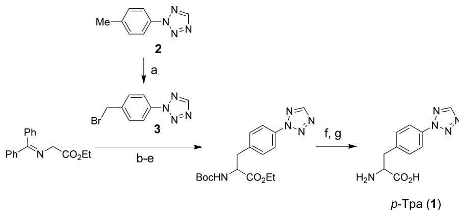
Scheme 1. Synthesis of p -(2-Tetrazole)phenylalanine ( 1 ) a
