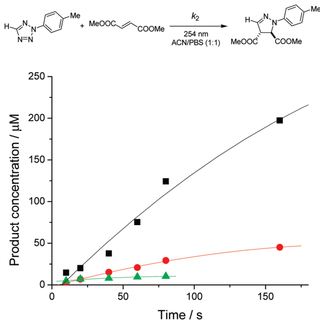
Figure 3. Time courses of the pyrazoline cycloadduct formation for the photoinduced cycloaddition reactions between 2-tolyltetrazole and dimethyl fumarate at three different concentrations: ■ = 1 mM 2-tolyltetrazole and 20 mM dimethyl fumarate; ● = 200 μM 2-tolyltetrazole and 20 mM dimethyl fumarate; ▲ = 200 μM 2-tolyltetrazole and 4 mM dimethyl fumarate.
