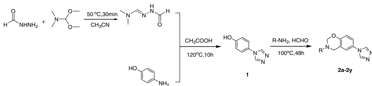
Fig. 1 Structure of compounds 1 , 2 , and 2a–y
