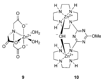
Figure 2. Complexes 9 and 10 representing receptor substructures.
