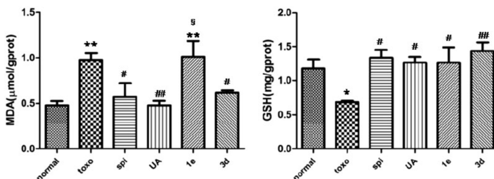
Figure 5. Effect of compounds on MDA and GSH levels in T. gondii -infected KM mice, * p < .05, ** p < .01 compared with normal group; # p < .05, ## p < .01 compared with toxо group; $ p < .05 compared with spi group.
