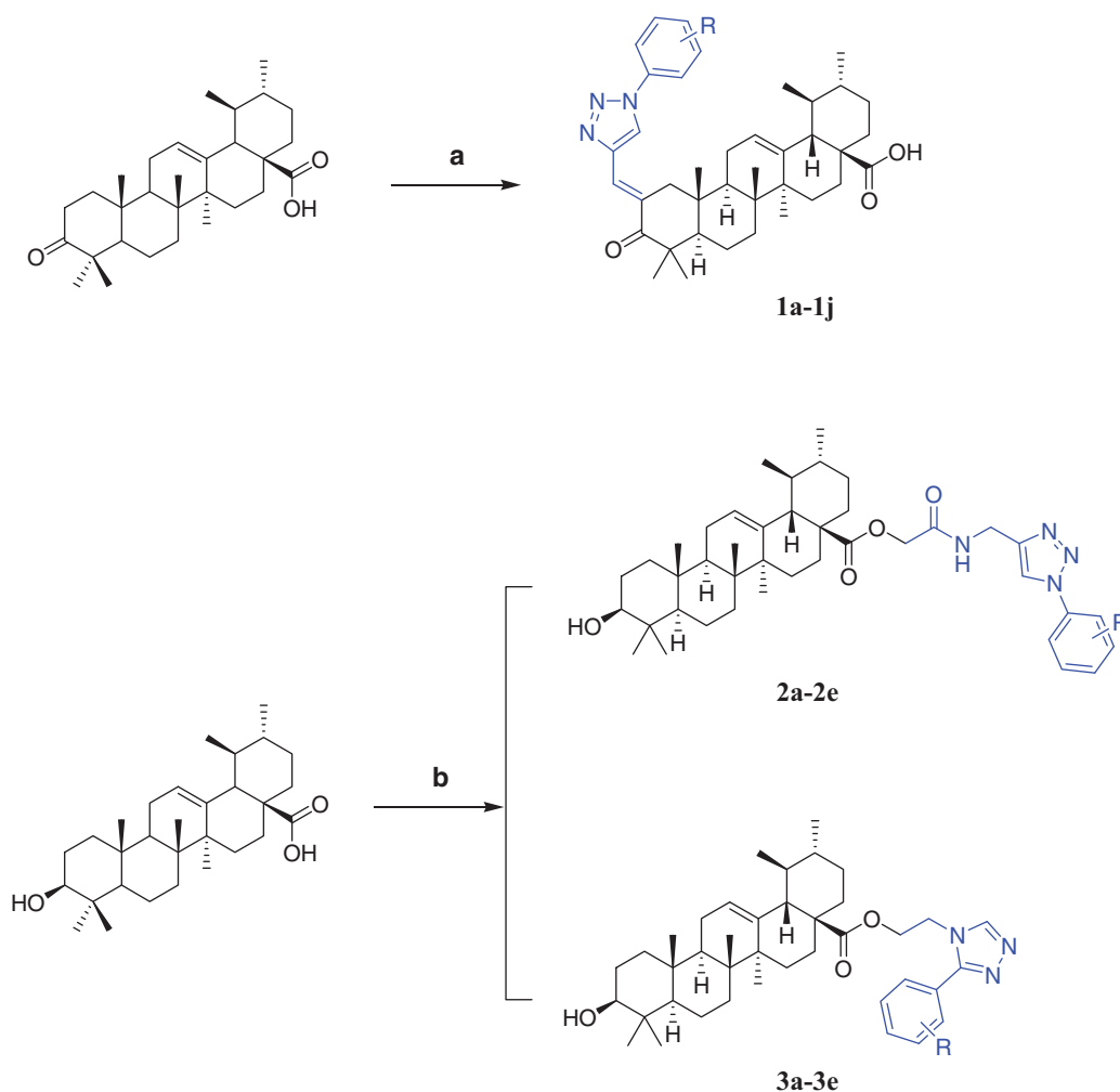
Scheme 2. Reagents and conditions: (a) 1a–1j , KOH, CH 3 CH 2 OH, 30 °C. (b) IIa–IIe , IIIa–IIIe , K 2 CO 3 , CH 3 CN, 60 °C.
