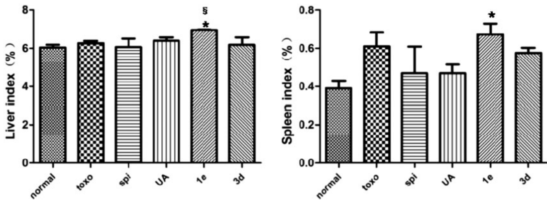
Figure 3. Effect of compounds on liver and spleen weights in T. gondii -infected KM mice, * p < .05 compared with normal group; $ p < .05 compared with spi group.
