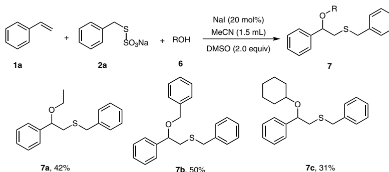
Scheme 5 Reagents and conditions: 1a (0.30 mmol), 2 (0.45 mmol), 6 (100 \mu\text{L} ), \text{H}_2\text{O} (0.60 mmol), NaI (20 mol%), 9 h in air. Yields are for the isolated products.
