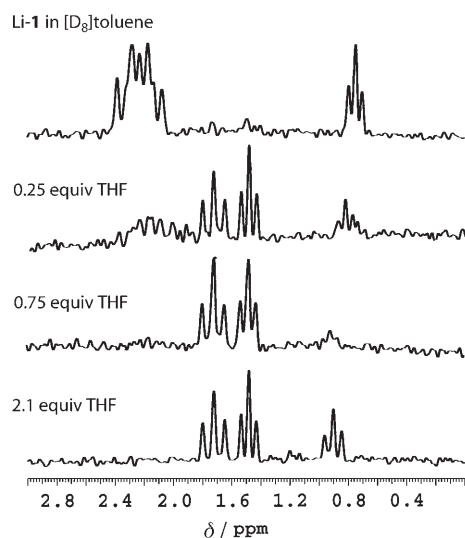
Figure 1. ^6\text{Li} NMR spectra of a THF titration of a solution of Li-1 in [\text{D}_8]\text{toluene} at -90^\circ\text{C} . In pure toluene, Li-1 exists as an oligomer, however, upon addition of a small amount of THF, two triplets from the nonequivalently solvated (\text{Li-1})_2 appear at \delta=1.5 ( J=3.8 Hz) and 1.7 ppm ( J=5.7 Hz). Upon further addition of THF, these signals are eventually replaced by a single triplet of the equivalently solvated (\text{Li-1})_2 at \delta=0.9 ppm ( J=4.2 Hz).
