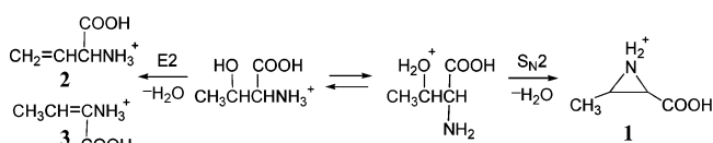
Scheme 4. Alternative Mechanisms for Side-Chain Water Loss
