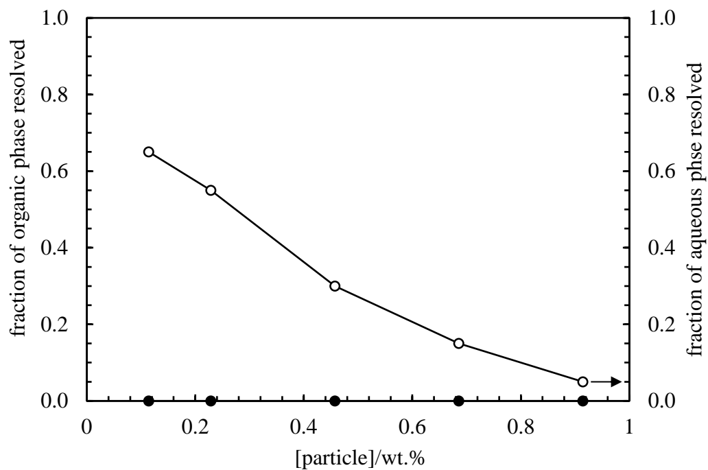
Figure 5. Fraction of aqueous (empty circles) and organic (filled circles) phase resolved from the o/w emulsions in Figure 4(a) prepared with different concentrations of 65% SiOH silica particles 1 month after preparation.
