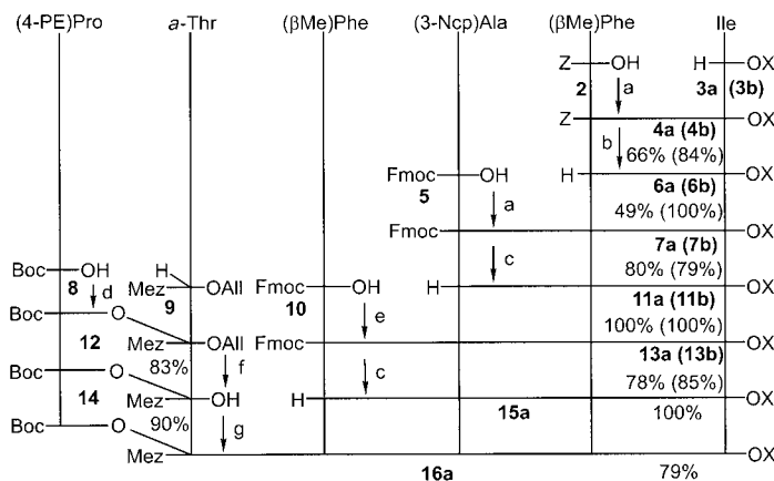
Scheme 1. Synthesis of the acyclic precursor 16a to the hexapeptolide fragment of hormaomycin 1 . a) EDC, HOAt, DIEA, 2,4,6-collidine, CH 2 Cl 2 , 0→20°C, 14 h; b) H 2 , Pd/C, EtOAc, 20°C, 40 min; c) 50% Et 2 NH/MeCN, 20°C, 1 h; d) EDC, 4-pyrrolidinopyridine, CH 2 Cl 2 , 0→20°C, 24 h; e) EDC, HOAt, 2,4,6-collidine, DMF, 0→20°C, 14 h; f) [Pd(PPh 3 ) 4 ], N -methylaniline, DME, 20°C, 1 h; g) HATU, HOAt, DIEA, 2,4,6-collidine, CH 2 Cl 2 , 0→20°C, 24 h. DCPM=dicyclopropylmethyl, All=allyl, Fmoc=9-fluorenylmethyloxycarbonyl, DIEA= N,N -diisopropylethylamine, EDC= N '-(3-dimethylaminopropyl)- N -ethylcarbodiimide hydrochloride, HATU= O -(7-azabenzotriazole-1-yl)- N,N,N',N' -tetramethyluronium hexafluorophosphate, HOAt=7-aza-1-hydroxybenzotriazole, MeZ= p -methylbenzyloxycarbonyl, MOM=methoxymethyl; X=MOM (or DCPM).
