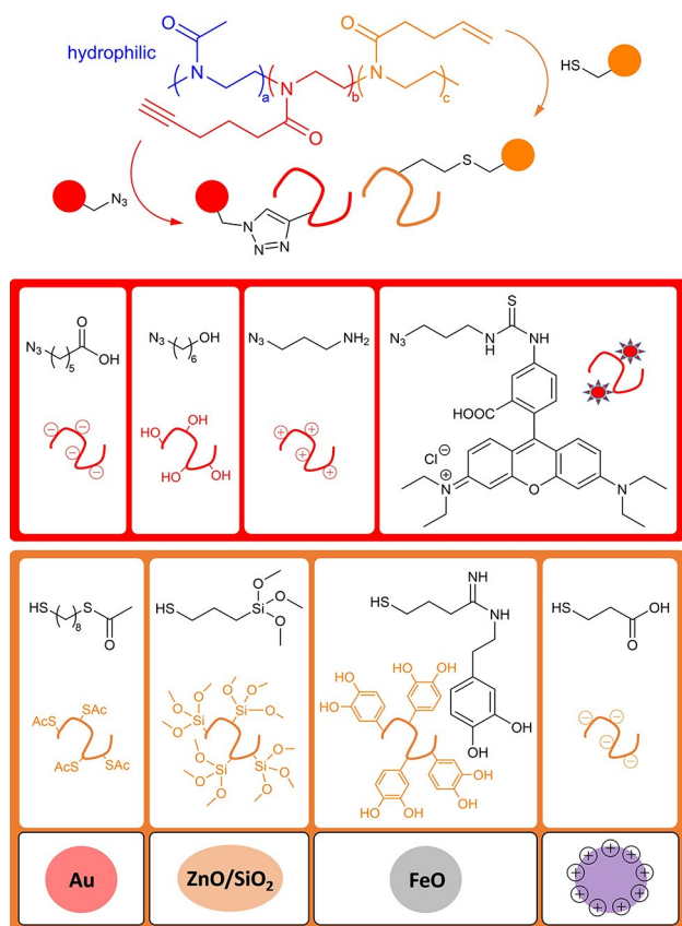
Figure 1. Schematic representation of the modular toolkit representing the orthogonal post-polymerization modification of a poly(2-oxazoline)-based triblock copolymer PMeOx-PPentynOx-PButenOx via azide-alkyne cycloaddition (CuAAC) and thiol-ene (TE) click reaction as well as potential systems for nanotechnological application.
