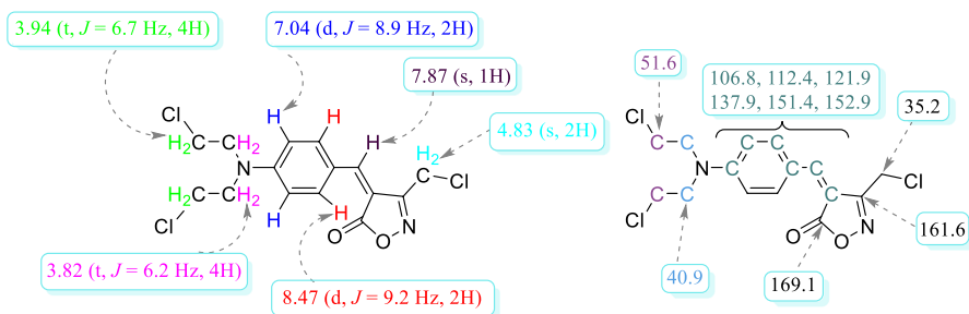
Fig. 4 1 H and 13 C NMR chemical shifts of heterocyclic compound 4ad
