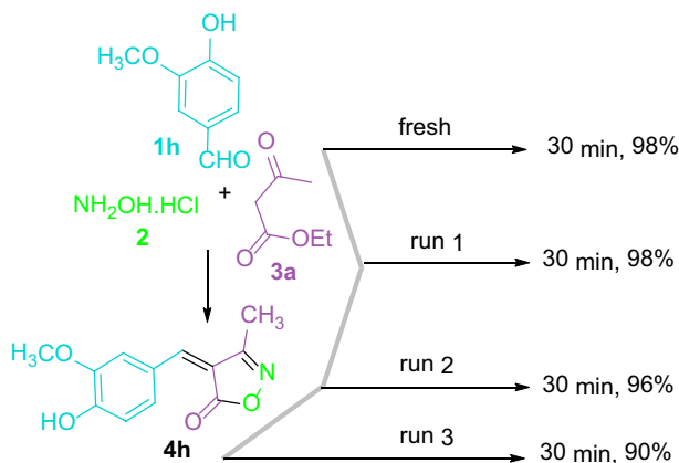
Fig. 5 Reusability of the catalyst
