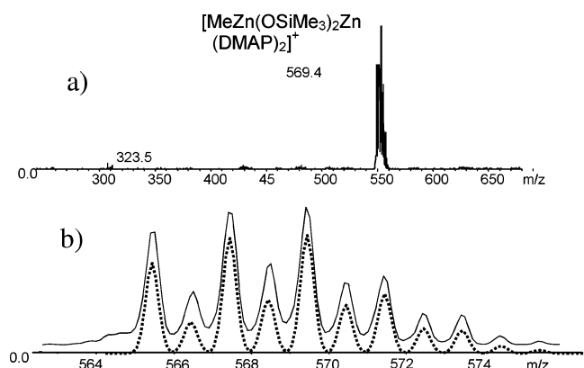
Figure 3. (a) ESI(+)-MS (CapEx 98.5 V) of the samples taken from the reaction mixture of 3 and \text{B}(\text{C}_6\text{F}_5)_3 in the presence of DMAP in THF. (b) Calculated (····) and experimental pattern for [\text{MeZn}(\text{OSiMe}_3)_2\text{Zn}(\text{DMAP})_2]^+ , 3 .
