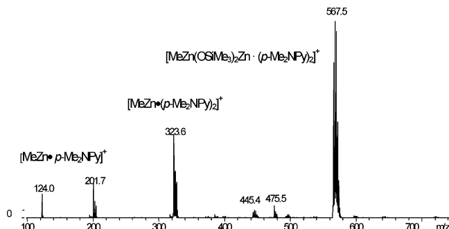
Figure 4. a. ESI(+)-MS (CapEx 113.5 V) of the samples taken from the reaction mixture of 1b and \text{B}(\text{C}_6\text{F}_5)_3 in the presence of DMAP in THF.
