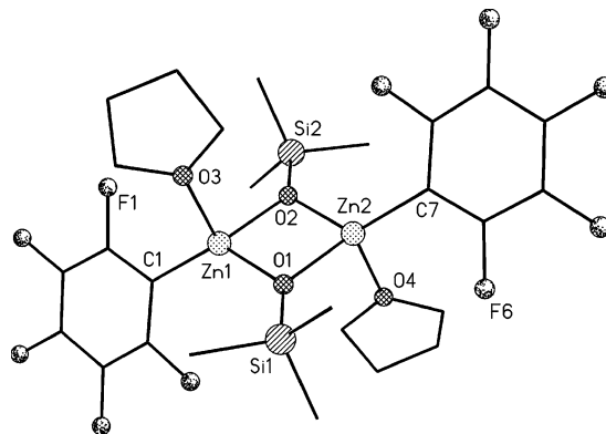
Figure 5. Molecular structure of [(\text{Me}_3\text{SiO})\text{ZnC}_6\text{F}_5(\text{thf})]_2 , 4 . The hydrogen atoms are omitted for clarity. Selected distances [Å] and angles [deg]: Zn(1)–O(1) 1.967(2), Zn(1)–O(2) 1.966(3), Zn(2)–O(1) 1.963(3), Zn(2)–O(2) 1.966(2), Zn(1)–Zn(2) 2.8768(9), O(1)–Zn(1)–O(2) 85.87(10), O(1)–Zn(2)–O(2) 85.9(1), Zn(1)–O(1)–Zn(2) 94.1(1), Zn(1)–O(2)–Zn(2) 94.0(1).
