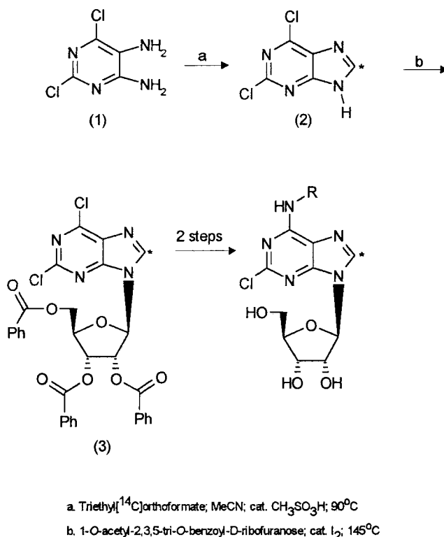
Scheme 1 Synthetic scheme for the preparation of 2-chloro-[8-purine- 14 C] nucleosides.
