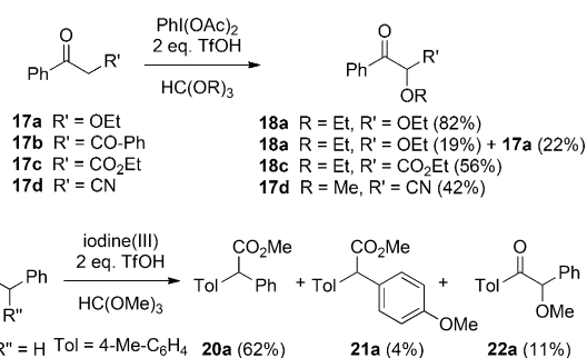
Scheme 5. Substituted substrates for the rearrangement reaction.
