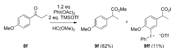
Scheme 2. Rearrangement and formation of diaryliodonium salt 9ff .
