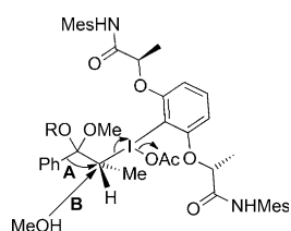
Figure 2. Intermediate 12 ( R=H, Me ).
