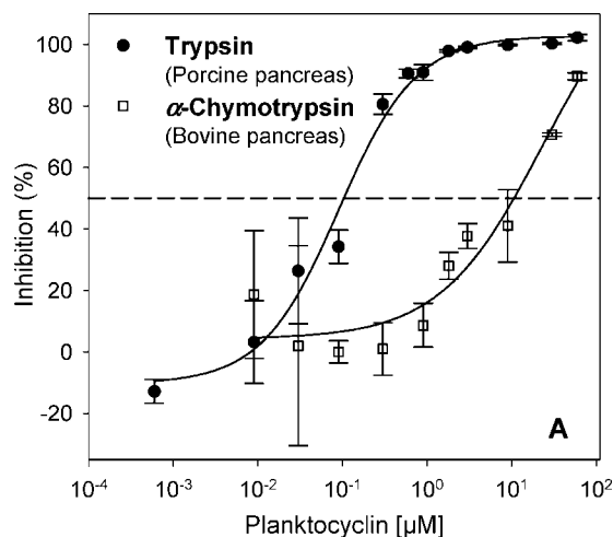
Figure 3. Planktocyclin concentration inhibition curves for trypsin ( R^2 = 0.996 ; P < 0.0001 ) and \alpha -chymotrypsin ( R^2 = 0.936 ; P = 0.226 ). Mean values of 3 replicates and standard deviation.
