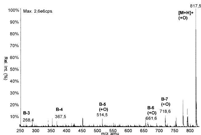
Figure 2. Mass fragmentation of planktocyclin sulfoxide and assignment of fragments.
