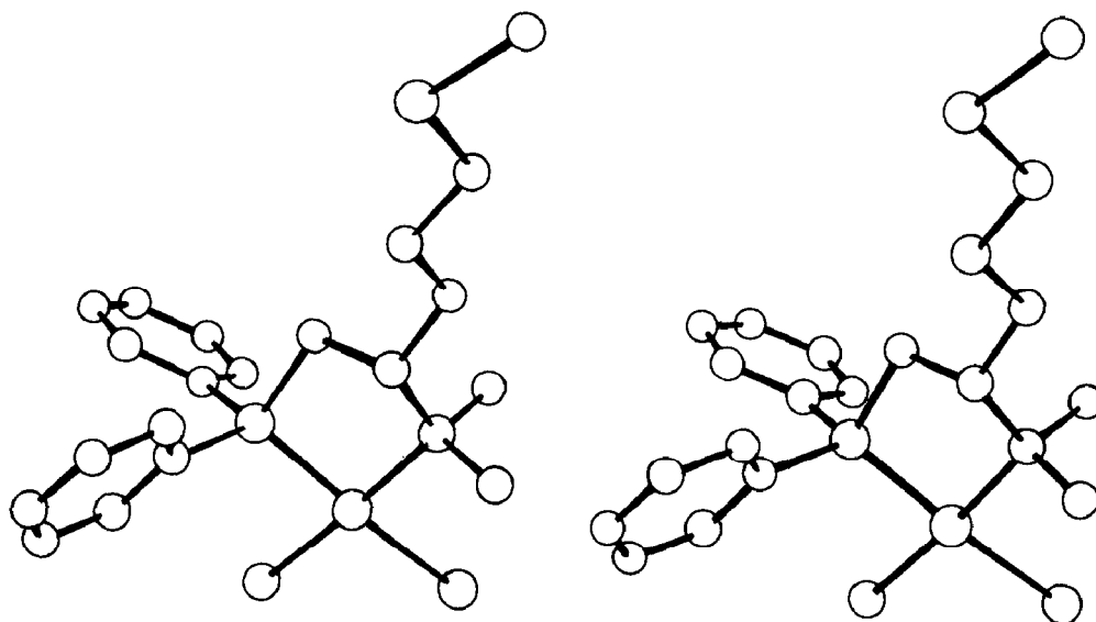
Fig. 4. Stereoplot of complex 4m ·PdCl 2 .
