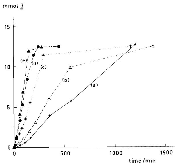
Fig. 5. Rate of formation of 3 in the presence of ligand 4m and varying amounts of ZnBr 2 . The maximum theoretical yield of 3 is 12.5 mmol. The code is (a) 0 mol% ZnBr 2 (rot. 3 +3.60°), (b) 0.13 mol% ZnBr 2 (rot. 3 +2.20°), (c) 1.0 mol% ZnBr 2 , (d) 11.5 mol% ZnBr 2 (rot. 3 -1.83°), (e) 200 mol% ZnBr 2 (rot. 3 -3.95°). If not reported, the rotation of 3 obtained at the end of the reaction was not measured.
