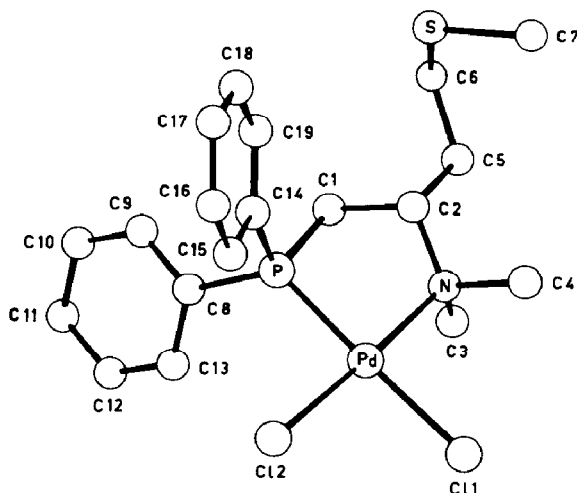
Fig. 1. Single molecule of complex 4h \cdot \text{PdCl}_2 with atom numbering scheme.
