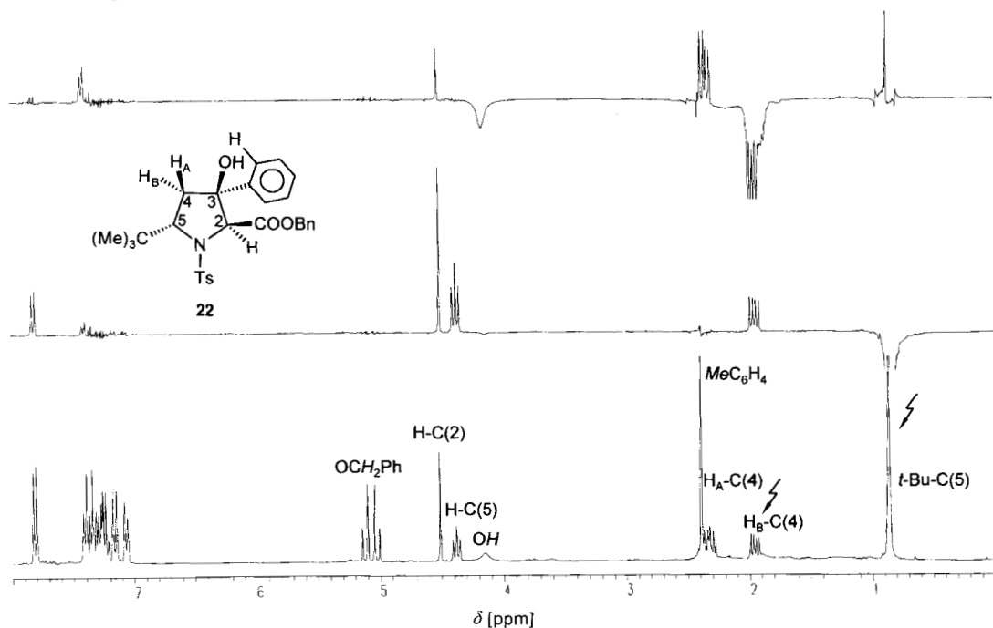
Fig. 2. ^1\text{H} -NMR Spectrum, NOE difference spectra and configuration of 22
