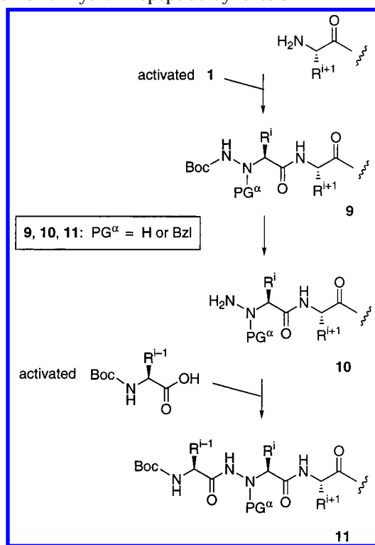
Scheme 2. Hydrazinopeptide Synthesis
