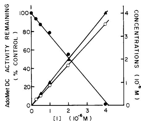
Figure 1. AdoMetDC inactivation (●), consumption of 1 (▲), and formation of 5'-(methylamino)-5'-deoxyadenosine (○) as a function of the initial concentrations of 1 . AdoMetDC (final concentration: 4 \mu\text{M} ) was incubated at 37 °C with various concentrations of 1 between 0 and 4 \mu\text{M} . After a 10-min incubation, two aliquots were withdrawn in parallel: (1) 5- \mu\text{L} aliquots, which were diluted in 295 \mu\text{L} of 50 mM HEPES buffer (pH 7.4), 50 \mu\text{L} of this mixture serving to measure enzyme activity remaining; 7 (2) 25- \mu\text{L} aliquots, to which was added 5 \mu\text{L} of 0.05 N \text{HClO}_4 to halt the reaction. Reversed-phase HPLC analysis of 1 and 5'-(methylamino)-5'-deoxyadenosine was performed after injection of 20 \mu\text{L} of these mixtures. 13
