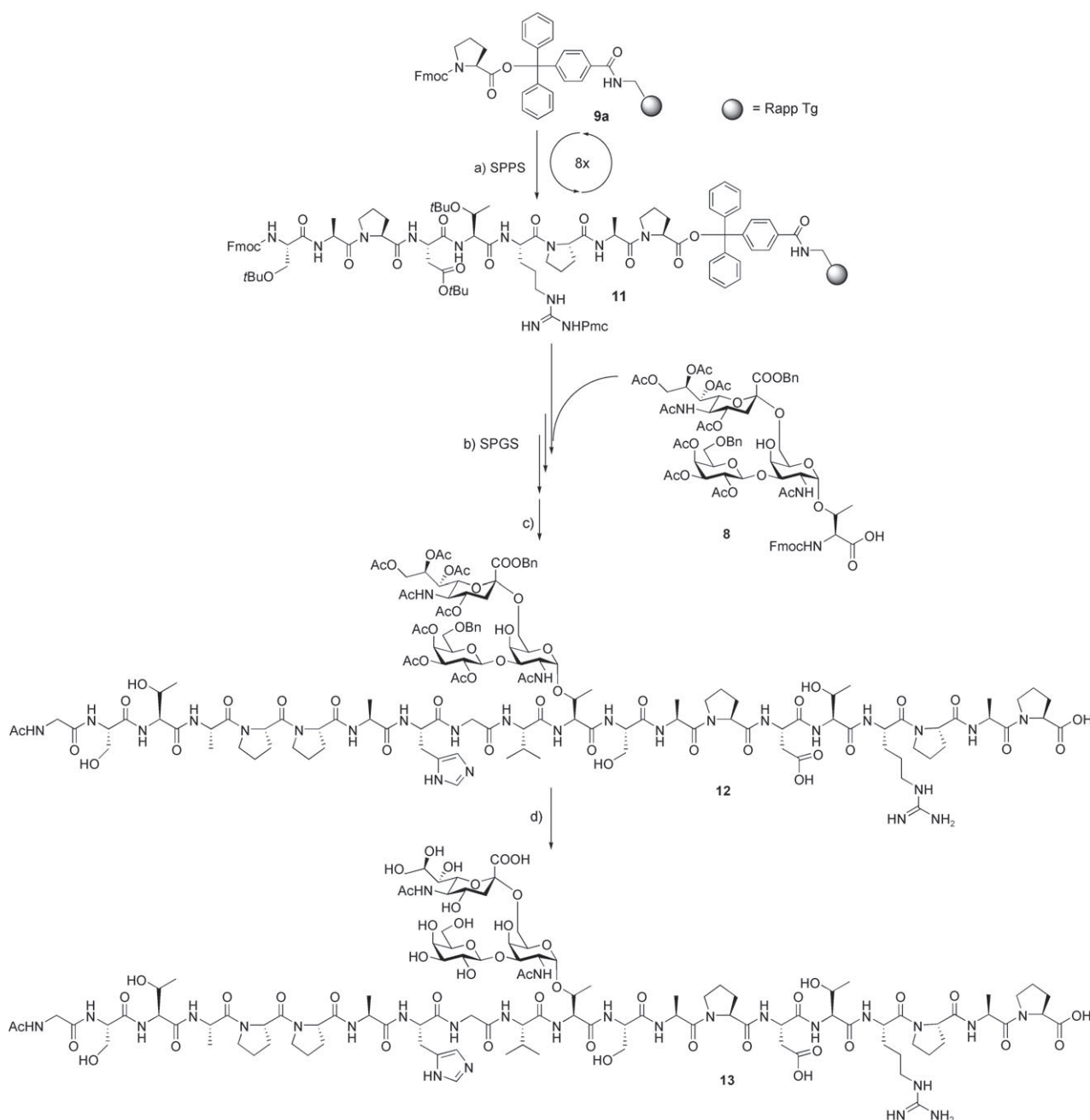
Scheme 3. a) Solid-phase peptide synthesis (SPPS): Fmoc removal (20% piperidine/NMP); coupling (steps 1–8: 1 mmol Fmoc-AA-OH, HBTU/HOBt/DIPEA, DMF; capping: Ac 2 O, DIPEA, HOBt 4:1:0.12. Synthesis of (2,6)-sialyl-T glycoconjugate 13 from MUC1: b) solid-phase glycopeptide synthesis (SPGS): Fmoc removal (20% piperidine/NMP); coupling step 9: 1.7 equiv 8 , HATU/HOAt/NMM, DMF, 4 h; steps 10–19: 1 mmol Fmoc-AA-OH, HBTU/HOBt/DIPEA, DMF; capping: Ac 2 O, DIPEA, HOBt 4:1:0.12; c) TFA/TIS/H 2 O 15:0.9:0.9, 2 h, 44% based on the pre-loaded resin 9a ; d) i) H 2 , 5% Pd/C, MeOH, 20 h, ii) NaOMe/methanol, pH 9.5, 55% over two steps. HATU = O -(7-aza-benzotriazole-1-yl)- N,N,N',N' -tetramethyluronium hexafluorophosphate, HBTU = O -(1 H -benzotriazol-1-yl)- N,N,N',N' -tetramethyluronium hexafluorophosphate, HOAt = N -hydroxy-7-azabenzotriazole, HOBt = N -hydroxybenzotriazole; NMM = N -methylmorpholine; TIS = triisopropylsilane; Pmc = 2,2,5,7,8-pentamethylchroman-6-sulfonyl.
