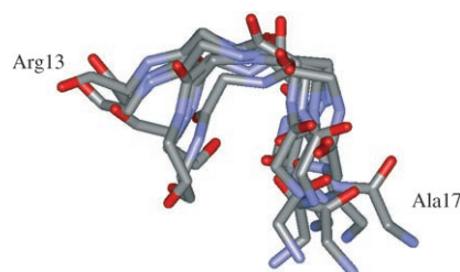
Figure 5. APDTR sequence of glycopeptide 13 exhibits a turn-like structure.
