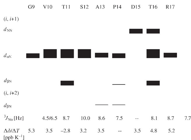
Figure 2. ROE connectivities, ^3J_{N\alpha} and temperature coefficients for glycopeptide 13 . The line thickness corresponds to the ROE intensity. In the case of proline, NH refers to \delta protons.
