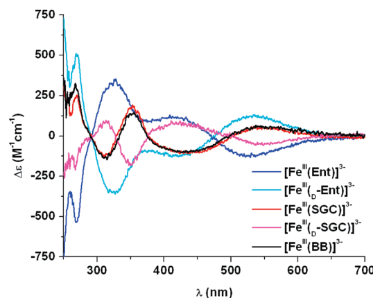
Figure 3. Circular dichroism spectra of the studied ferric complexes ( [\text{FeL}] = 0.1 \text{ mM} , pH 7.4, 1 cm path, 25 °C).
