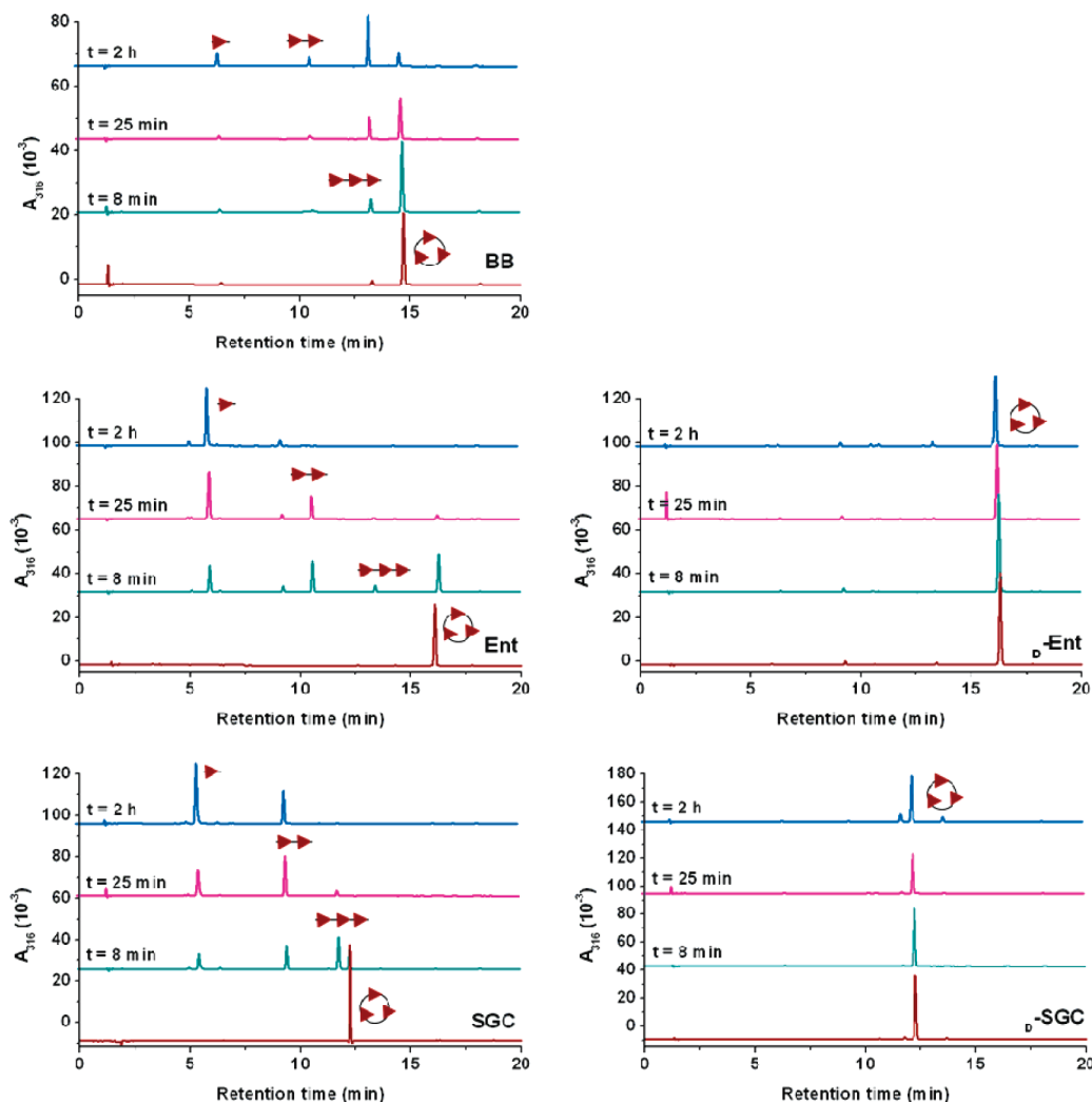
Figure 6. Reaction time courses of Bes-catalyzed hydrolysis of BB (top), Ent (middle left) and SGC (bottom left). The presence of Bes in solution did not affect D-Ent (middle right) and D-SGC (bottom right). Reaction aliquots were quenched at different time points and analyzed by HPLC. The assignment of the hydrolysis products is based on the corresponding mass spectrometry data (Figures S4–S6, Supporting Information), and the schematic representations of the hydrolysis products (cyclic trimer, linear trimer, dimer and monomer) are shown consistently with similar previous studies. 29
