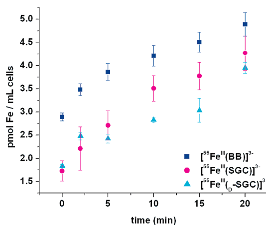
Figure 4. Iron transport mediated by [Fe III (BB)] 3- , [Fe III (SGC)] 3- , and [Fe III (D-SGC)] 3- in B. subtilis at 37 °C in iron-limited medium. Data presented are the average of three independent experiments for BB and SGC, and two independent experiments for D-SGC.
