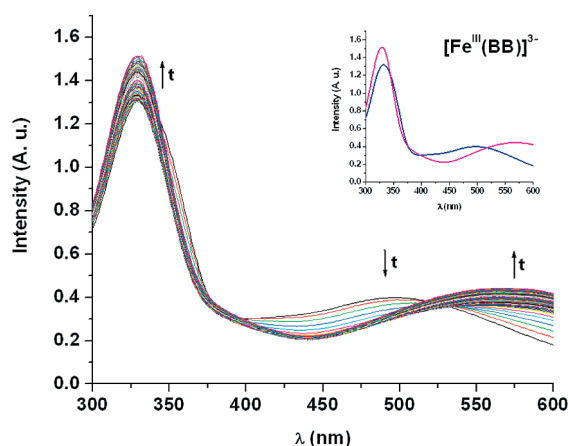
Figure 7. Bes-catalyzed hydrolysis of [\text{Fe}^{\text{III}}(\text{BB})]^{3-} to [\text{Fe}^{\text{III}}(2,3\text{-DH-BGT})_3]^{3-} followed by UV–vis spectroscopy ( [\text{Fe}(\text{BB})] = 100 \mu\text{M} , [\text{Bes}] = 1 \mu\text{M} , 75 mM HEPES, pH 7.5, 25 °C, 1 cm cell). The inset shows the spectra at t = 0 h (blue) and t = 12 h (pink).
