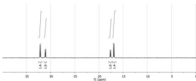
Fig. 9 ^{31}\text{P} -NMR spectra of the organic phase of the ELLE of DL-Cys-Na, taken at T = -40\text{ }^{\circ}\text{C} . Conditions ELLE: host = \text{PdCl}_2((S)\text{-BINAP}) , [host] = 10.0 mM, [substrate] = 20.0 mM, T = 6\text{ }^{\circ}\text{C} .
