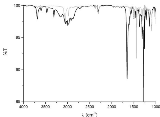
Fig. 12 FTIR spectra of \text{PdCl}_2((S)\text{-BINAP}) (grey) and \text{PdCl}((S)\text{-BINAP})(\text{D-Trp}) (black).
