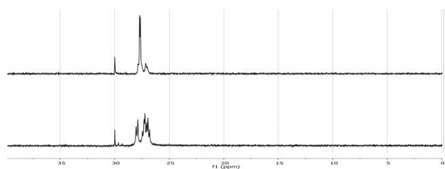
Fig. 8 ^{31}\text{P} -NMR spectra of the organic phase of the ELLE of DL-Trp-Na, taken at T = -40\text{ }^{\circ}\text{C} (bottom) and +20\text{ }^{\circ}\text{C} (top). Conditions ELLE: host = [\text{PdCl}_2((S)\text{-BINAP})] , [host] = 10.0 mM, [substrate] = 20.0 mM, T = 6\text{ }^{\circ}\text{C} .
