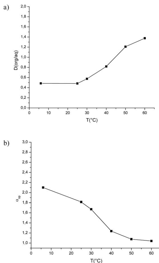
Fig. 5 The relation between temperature and the distribution (a) and the \alpha_{op} (b) of the ELLE of Trp. Conditions: \text{PdCl}_2((S)\text{-BINAP}) (1.0 mM), Trp-Na (2.0 mM), n-octanol, dd. water. Lines are a guide to the eye.
