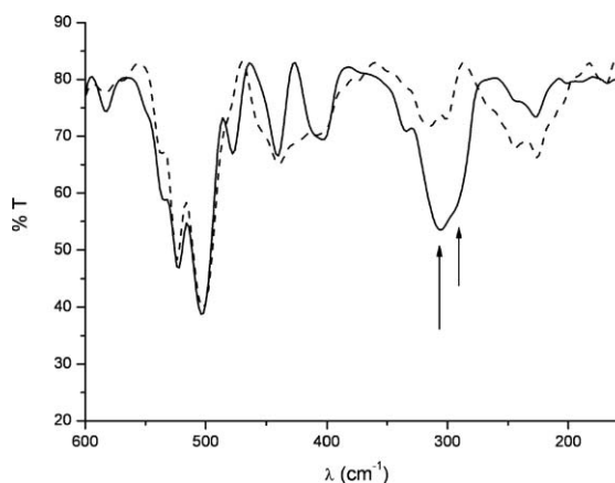
Fig. 14 FT-FIR spectra of \text{PdCl}_2((S)\text{-BINAP}) (black) and \text{PdCl}((S)\text{-BINAP})\text{-D-Trp} (dashed).
