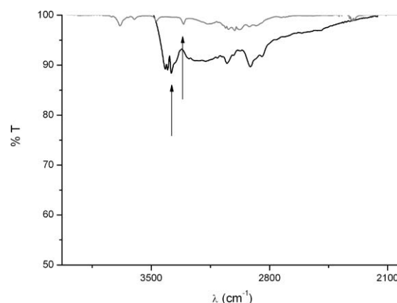
Fig. 13 FTIR spectra of \text{PdCl}((S)\text{-BINAP})(\text{D-Trp}) (grey) and Trp-Na (black). Arrows indicate absorption bands assigned to the stretching vibrations of the primary amine.
