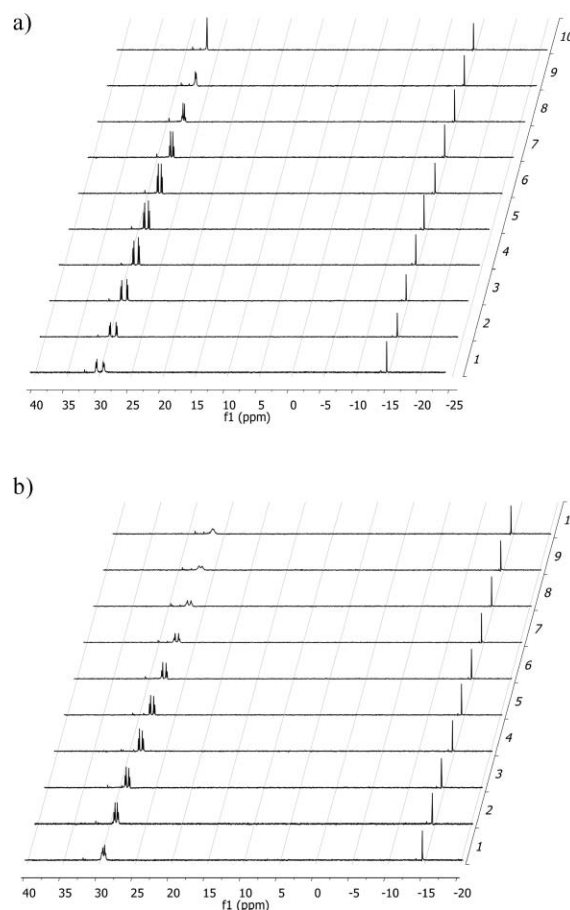
Fig. 7 Temperature dependent studies on the \text{PdCl}_2((S)\text{-BINAP}) -D-Trp (a) and \text{PdCl}_2((S)\text{-BINAP}) -L-Trp (b) complex. Spectra 1–10 represent T = -50^\circ\text{C} to +40^\circ\text{C} at 10^\circ\text{C} intervals.
