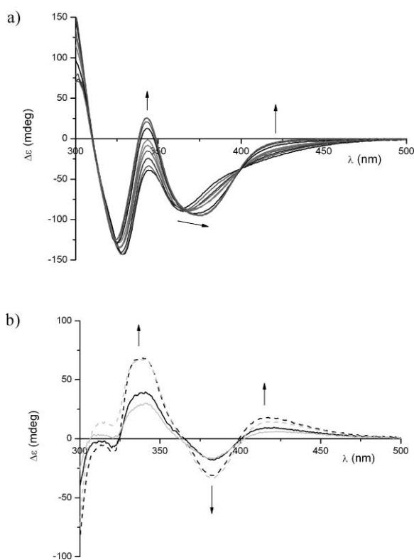
Fig. 11 CD spectra of \text{PdCl}_2((S)\text{-BINAP}) upon titration of D-Trp (0.0–10.0 mM) (a) and CD differential spectra (b) of D-Trp (black) and L-Trp (grey) at 1.0 mM (solid) and 10.0 mM (dashed).
