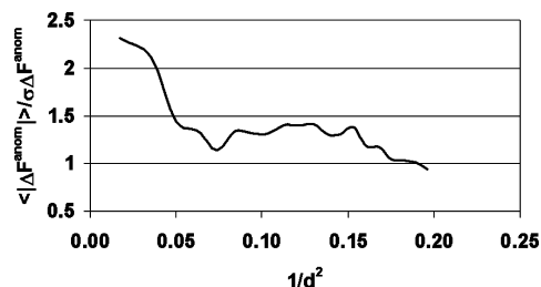
Figure 1. Plot of \langle \Delta F_{\text{anom}} / \sigma \Delta F_{\text{anom}} \rangle versus 1/d^2 , where d is the interplanar spacing, for Cs-ACN. The diffraction anomalous signal is above one across the whole resolution range.
