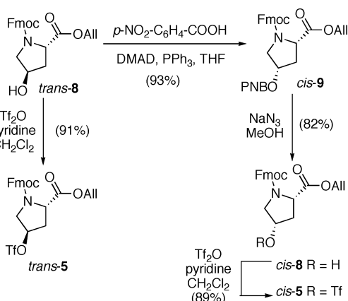
Scheme 5. Synthesis of Hyp and hyp Derivatives
