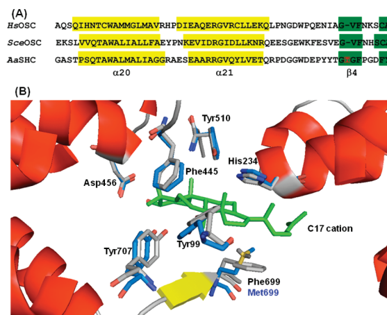
Figure 1. (A) Partial sequences alignment among HsOSC, SceERG7, and AaSHC. (B) The superimposed homology models of SceERG7 and SceERG7 F699M complexed with protosteryl C-17 cation.
