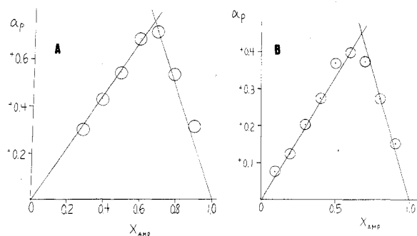
Figure 4. Job's method plot of 5'-AMP and \text{Zn(phen)}_3^{2+} (23 °C): (A) pH 5.9; (B) pH 7.3.
