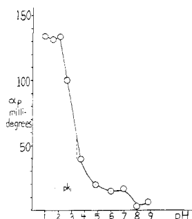
Figure 2. pH dependence of \text{Ni(phen)}_3^{2+} ( l -malic acid data from ref 4).
