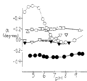
Figure 1. The pH dependence of the optical rotations of nucleosides, nucleotides, and related compounds: O, 5'-AMP + \text{Zn(phen)}_3^{2+} ; ●, 5'-AMP alone; □, ribose phosphate + AMP; △, ribose phosphate alone; ▼, adenosine + \text{Zn(phen)}_3^{2+} ; ▽, adenosine alone.
