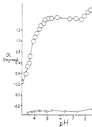
Figure 3. pH dependence of 3',5'-c-AMP (squares) and of \text{Zn(phen)}_3^{2+} (circles).
