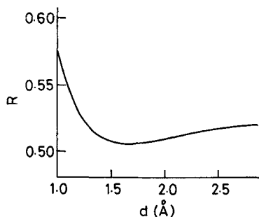
Fig. 10. The dependence of agreement factor ( R ) on the distance between \text{Yb}^{3+} and carbonyl \text{O} -atom ( d )
