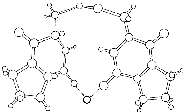
Fig. 11. Proposed conformation of \text{S,S}' -bis(cyclo(hemiCys-Pro))/metal ion complex
