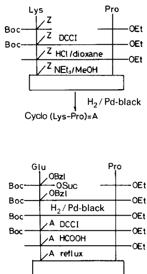
Fig. 1. Synthetic route of cyclo(Lys-Pro) cyclo(Glu-Pro) ( bis(I) )
