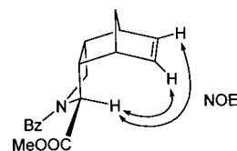
Fig. 2. NOE Relationships of Diels–Alder Adduct 11
