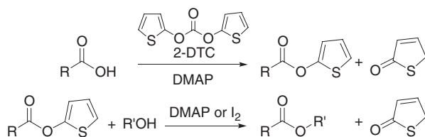
Scheme 1. Esterification of carboxylic acids with alcohols using 2-DTC promoted by DMAP and iodine.
