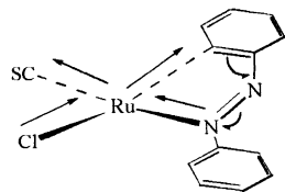
Fig. 4. Numbering scheme for ^{13}\text{C} -NMR data.
