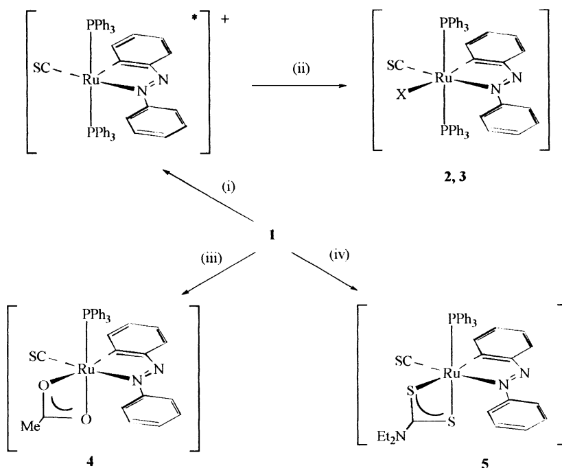
Scheme 1. (i) \text{AgNO}_3 , \text{CH}_2\text{Cl}_2 , \text{EtOH} , \text{H}_2\text{O} ; (ii) \text{NaX} ( \text{X} = \text{Br}, \text{I} ); (iii) \text{AgOC}(\text{O})\text{Me} , \text{CH}_2\text{Cl}_2 ; (iv) \text{NaS}_2\text{CNET}_2 \cdot 2\text{H}_2\text{O} , \text{CH}_2\text{Cl}_2 , \text{EtOH} , \text{H}_2\text{O} .
