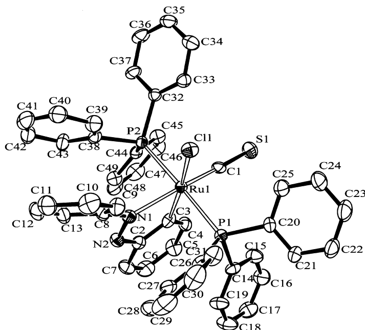
Fig. 1. ORTEP representation of 1 showing the atomic numbering scheme.
