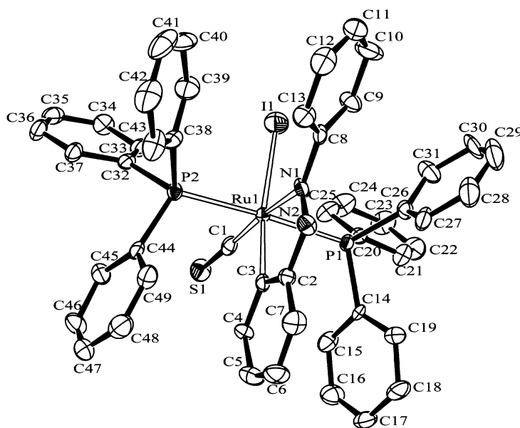
Fig. 2. ORTEP representation of 3 showing the atomic numbering scheme.
