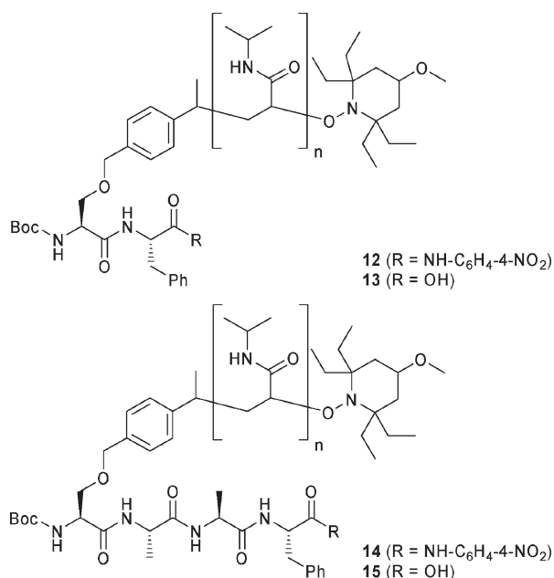
Fig. 4 Alkoxyamines 12 and 14 used in the enzymatic hydrolysis to yield 13 and 15 .
