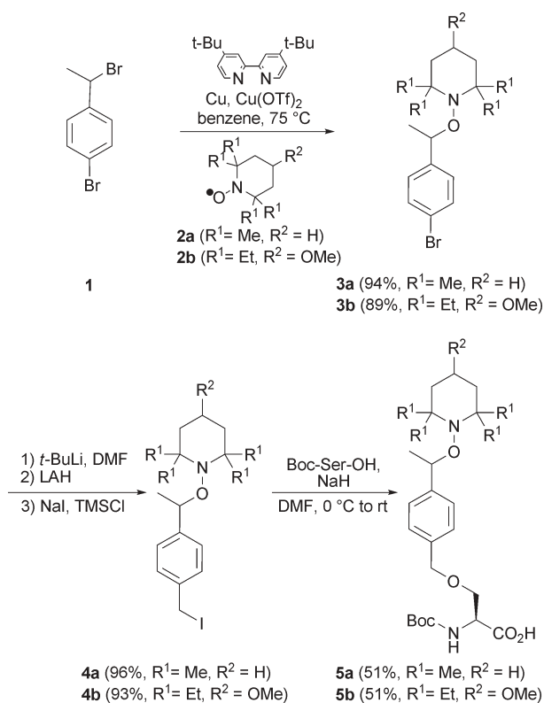
Scheme 1 Synthesis of alkoxyamines 5a and 5b .
