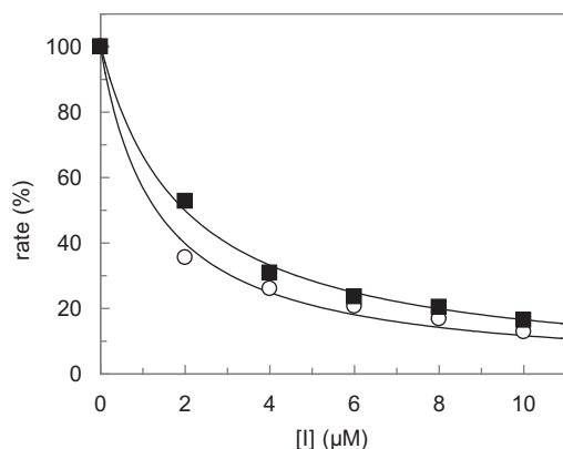
Figure 2. Inhibition of porcine CEase by compounds 10f (open circles) and 10l (closed squares). Data are means of duplicate measurements. Non-linear regression according to the equation v = v_0/(1 + ([I]/IC_{50})^x) gave values IC_{50} = 1.33 \pm 0.12 \mu M and IC_{50} = 1.98 \pm 0.11 \mu M , respectively.
