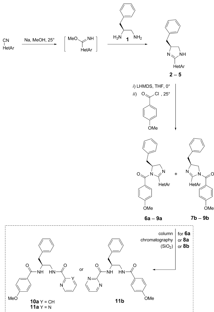
Scheme. Synthesis Pathway to Benzyl-Imidazolines 2–5 and 6–9 and Their Observed Ring Opening during Column Chromatography
