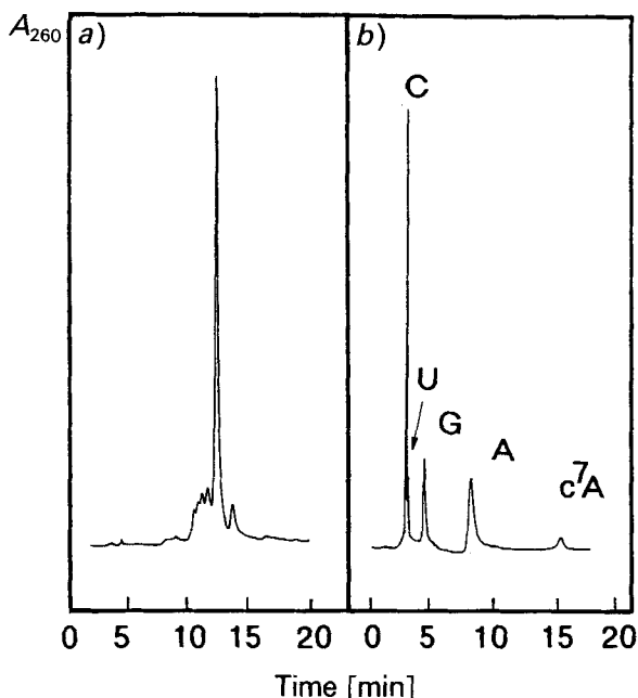
Fig. 2. HPLC Profiles of G-C-G-C-C-G-A-c^7A-A-C-U-C-C-C ( [(c^7A)^{14}]E ; 11 ) obtained on a RP-18 column: a) crude oligomer after desilylation and desalting; b) after enzymatic hydrolysis with snake-venom phosphodiesterase followed by alkaline phosphatase. Conditions, see Exper. Part.
