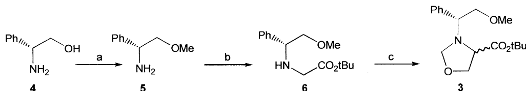
Scheme 1. Reagents and conditions: (a) (i) KH, THF; (ii) MeI, 77%; (b) BrCH 2 CO 2 tBu, K 2 CO 3 , MeCN, 73%; (c) (CH 2 O) n toluene, Δ, 87%
