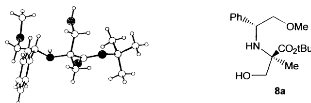
X ray structure of compound 8a
