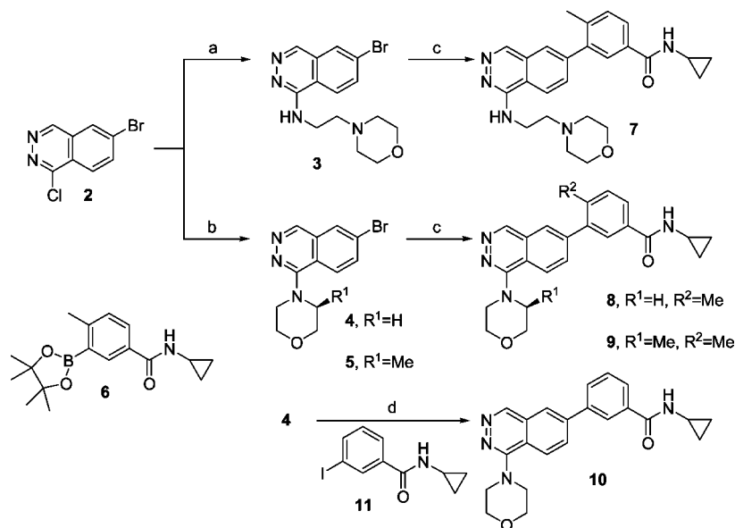
Scheme 1. Synthesis of 1-Aminophthalazines 7–10 a
