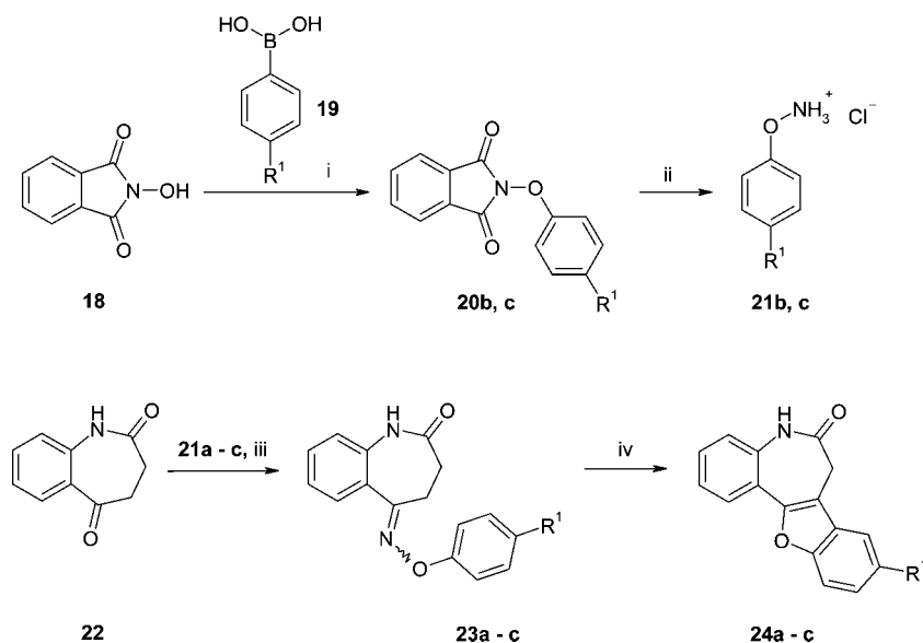
Scheme 4. Synthesis of 12-Oxapaullones 24 a
