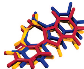
Figure 3. 1-Azakenpauillone ( 2a , blue), 2-azakenpauillone ( 13a , yellow), and 12-oxapauillone ( 24b , red) aligned by FlexX in the GSK-3β ATP binding site (generated from the PDB file 1Q3W.pdb). 34
