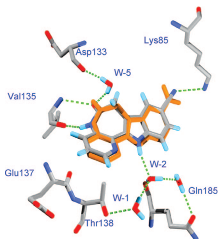
Figure 2. Alsterpauillone ( 1b ; light-brown, hydrogen atoms omitted) and 9-cyano-1-azakenpauillone ( 2b , atom color code) bound to the ATP binding site of GSK-3β. Hydrogen bonds involving 2b are indicated as green dashed lines. The pose of alsterpauillone is based on PDB file 1Q3W.pdb, 34 and the pose of 2b was generated using the FlexX module in Sybyl.
