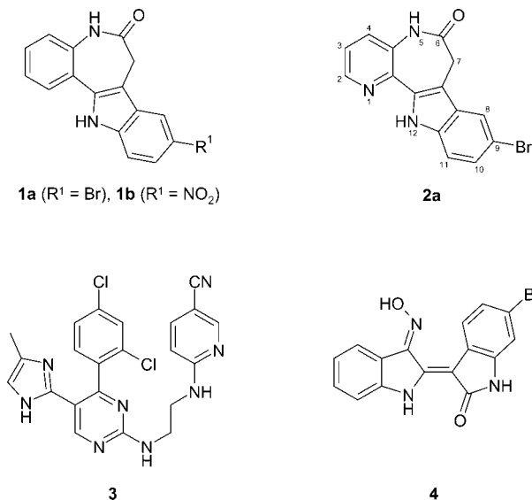
Figure 1. Structures of established GSK-3 inhibitors: kenpauillone ( 1a ), alsterpauillone ( 1b ), 1-azakenpauillone ( 2a ), CHIR99021 ( 3 ), and 6-bromoindirubin-3'-oxime (6BIO, 4 ).
