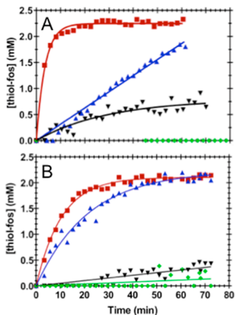
Figure 2. Time course of the FosB catalyzed-addition of BSH or L-Cys to fosfomycin in the presence of \text{Mg}^{2+} or Ni(II). Results for FosB SA and FosB BS are shown in panels A and B, respectively. Reactions were run at 25 °C in 20 mM HEPES (pH 7.0) with 4 mM fosfomycin and 0.5 \mu\text{M} enzyme in the presence of (■) 2 mM BSH and 10 \mu\text{M} Ni(II), (▲) 2 mM BSH and 1 mM \text{Mg}^{2+} , (▼) 2 mM L-Cys and 10 \mu\text{M} Ni(II), or (◆) 2 mM L-Cys and 1 mM \text{Mg}^{2+} .
