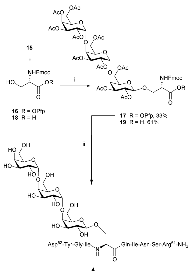
Scheme 2 Reagents, conditions and yields: i) \text{BF}_3 \cdot \text{Et}_2\text{O} , MeCN; ii) solid-phase peptide synthesis; then NaOMe, MeOH (28%, based on resin capacity).
