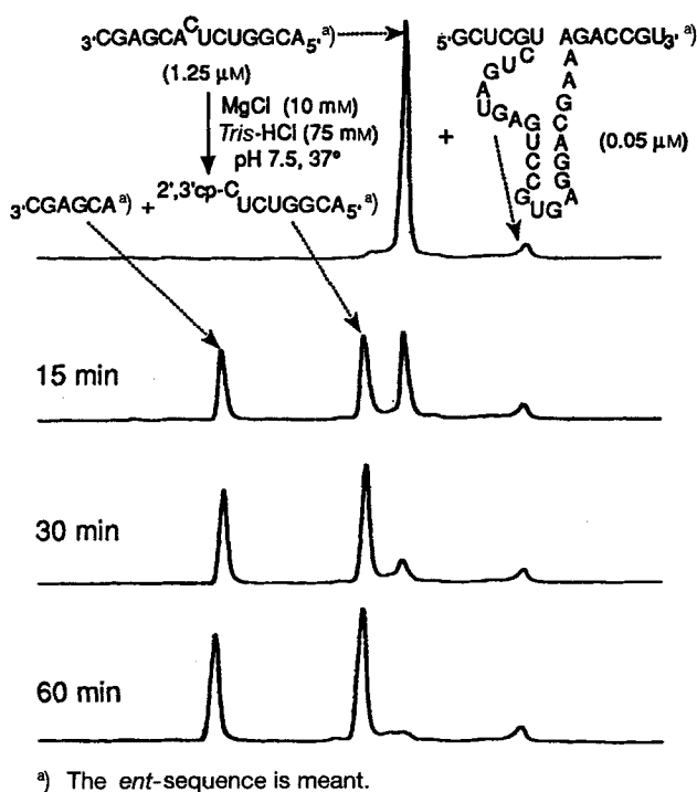
Fig. 4. Functional analysis of the 35mer ent -oligonucleotide Q. Its known function as catalyst in the selective cleaving of the tetradecamer sequence O was followed by ion-exchange HPLC (conditions, see Exper. Part ); the reaction was carried out according to [33] and could be completely reproduced. The identity of the two produced ent -oligonucleotides was unambiguously confirmed by coinjection with authentic samples (the octamer cyclophosphate sequence was synthesized from ent -oligonucleotide M under conditions described in [29]).
