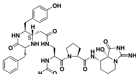
Pseudotheonamide A 1 ( 1 )
