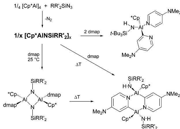
Scheme 6. Summary of the Reactions of [\text{Cp}^*\text{Al}]_4 with Trialkylsilyl Azides \text{RR}'_2\text{SiN}_3 and dmap
