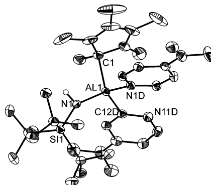
Figure 6. Molecular structure and atom-numbering scheme of compound 12 . Thermal ellipsoids are drawn at the 50% probability level. H atoms, except those attached to N, have been omitted for clarity. Selected bond lengths [ \text{\AA} ] and angles [ ^{\circ} ]: \text{Al1}-\text{N1} 1.829(2) , \text{Al1}-\text{N1D} 1.942(2) , \text{Al1}-\text{C1} 2.098(2) , \text{Al1}-\text{C12D} 2.004(2) , \text{N1}-\text{Si1} 1.725(2) ; \text{N1}-\text{Al1}-\text{N1D} 107.9(1) , \text{N1}-\text{Al1}-\text{C12D} 115.7(1) , \text{N1}-\text{Al1}-\text{C1} 109.3(1) , \text{N1D}-\text{Al1}-\text{C12D} 108.4(1) , \text{N1D}-\text{Al1}-\text{C1} 105.1(1) , \text{C12D}-\text{Al1}-\text{C1} 110.0(1) , \text{Al1}-\text{N1}-\text{Si1} 149.0(1) .
