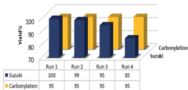
Fig. 8 The reusability results of the catalyst. Suzuki: 4-iodoanisole, carbonylation 4-iodotoluene as the substrates under the optimized conditions.
