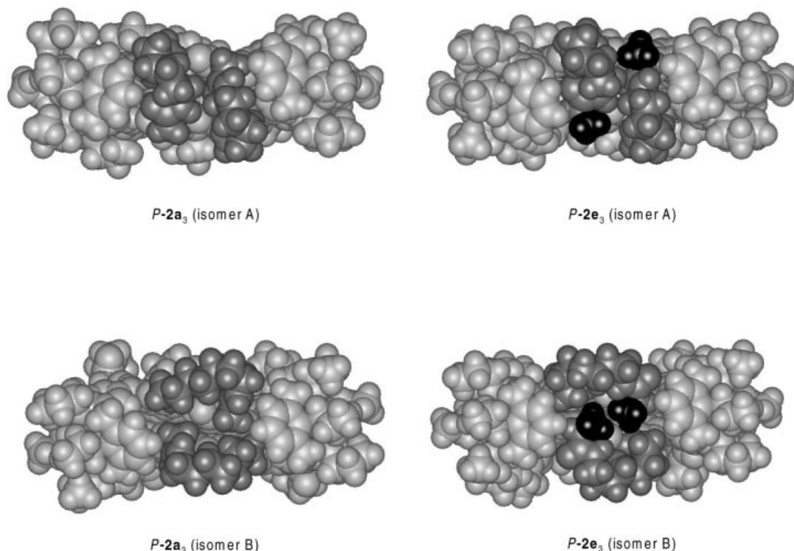
Figure 5. Gas-phase-minimized structures of both isomers (A and B) of assemblies 2a 3 , and 2e 3 ; these structures clearly illustrate the very different environments that the methyl ( 2e ) substituents experience in the two isomers
