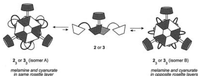
Scheme 2. Formation of two different isomers (A and B) for the self-assembly of the 3-component double-rosette assemblies 2_3 and 3_3
