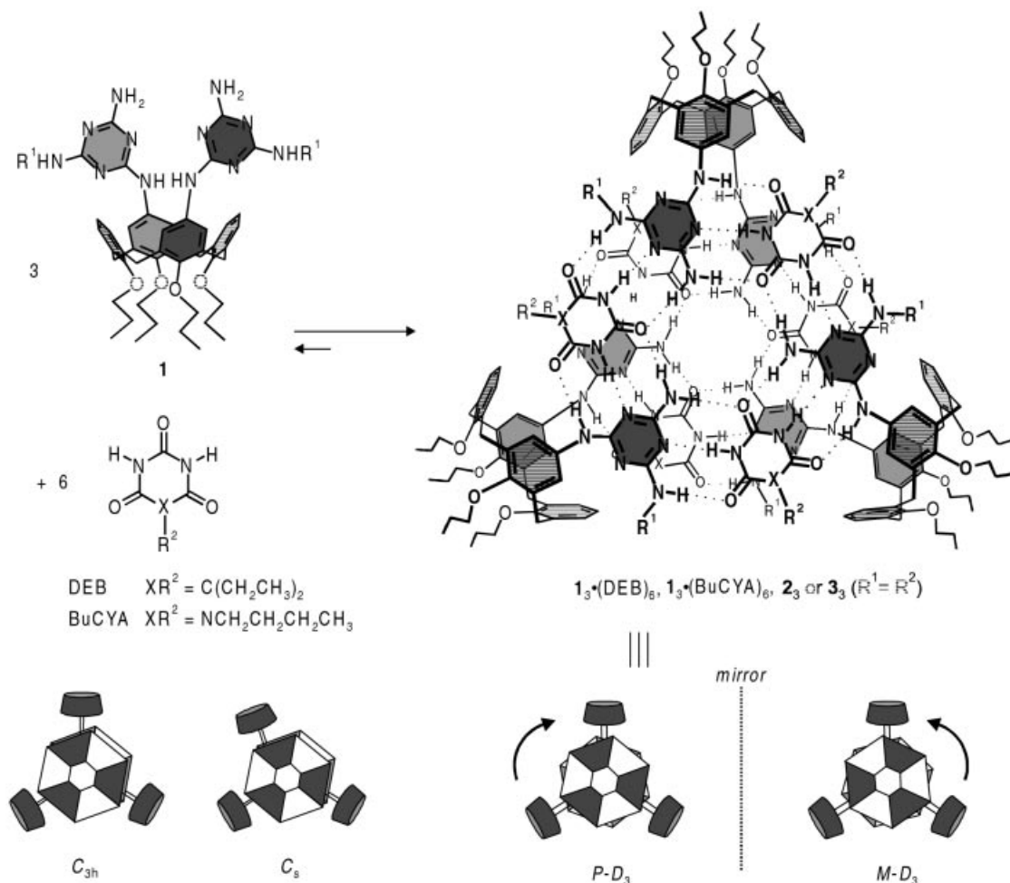
Figure 1. Molecular structure and schematic representations of the nine-component double rosette assemblies 1_3 \cdot (\text{DEB})_6 and 1_3 \cdot (\text{BuCYA})_6 and the three-component assemblies 2_3 and 3_3 , together with all possible isomeric conformations
