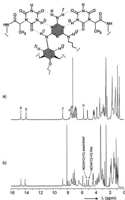
Figure 6. ^1\text{H} NMR spectra for double rosette assemblies 2\text{e}_3 in: a) \text{CDCl}_3/[\text{D}_6]\text{DMSO} (9:1), b) \text{CDCl}_3/[\text{D}_6]\text{DMSO} (45:55); the latter shows the coexistence of assembly 2\text{e}_3 and of free 2\text{e} , shown by two separate peaks for the \alpha\text{-CH}_2 of the cyanurate
