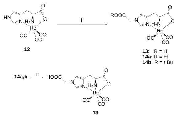
Scheme 5. i) Ethyl/ tert -butyl bromoacetate, \text{Cs}_2\text{CO}_3 , \text{CH}_3\text{CN} , 35 °C, 1.5 h, 90 %; ii) deprotection: ethyl ester: 0.5 M \text{LiOH}/\text{MeOH} (1:2), RT, overnight; tert -butyl ester: \text{TFA}/\text{CH}_2\text{Cl}_2 1:1, RT, 2 h.
