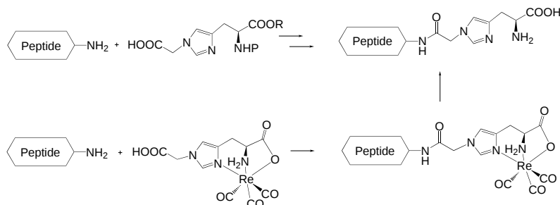
Scheme 1. Introduction of tripodal, \text{N}^\epsilon functionalized histidine into a biomolecule for labeling with [^{99m}\text{Tc}(\text{CO})_3]^+ .
