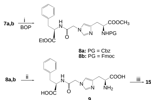
Scheme 3. i) H-Phe-OEt, BOP, \text{Et}_3\text{N} , \text{CH}_2\text{Cl}_2 , RT, 1.5–2.5 d, 74–90 %; ii) deprotection: Cbz: \text{H}_2 , Pd/C, \text{MeOH}/\text{H}_2\text{O}/\text{AcOH} (7:2:1), RT, 2 h; Fmoc: piperidine, RT, 30 min; ester: 0.5 M \text{LiOH}_{\text{aq}}/\text{MeOH} (1:2), RT, overnight; iii) [\text{Et}_4\text{N}]_2[\text{ReBr}_3(\text{CO})_3] , \text{H}_2\text{O} , RT, 19 h, 40–50 %.
