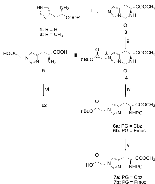
Scheme 2. i) 2 , \text{Im}_2\text{CO} , DMF, 70 °C, 6 h, 61 %; ii) bromoacetic tert -butyl ester, \text{CH}_3\text{CN} , reflux, 24 h; iii) 6 N HCl, reflux, 48 h; iv) 6a : BnOH, THF, reflux, 16 h, 62 % (from 3 in two steps); 6b : Fm-OH, \text{CH}_3\text{CN} , RT, 14 h, 55 % (from 3 in two steps); v) TFA/ \text{CH}_2\text{Cl}_2 1:1, RT, 2.5 h; vi) [\text{Et}_4\text{N}]_2[\text{ReBr}_3(\text{CO})_3] , \text{H}_2\text{O} , RT, 21 h, 68 % (from 3 in three steps).
