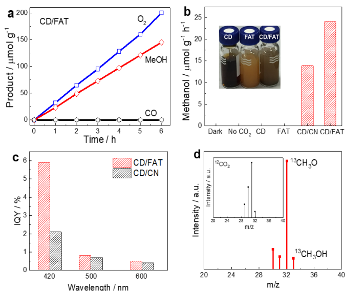
Figure 2. Photocatalytic \text{CO}_2 conversion to methanol. The photocatalytic activity of (a) CD/FAT measured under visible light ( \lambda > 420 \text{ nm} ). (b) Control experiments on CD, FAT, CD/CN. Inset: image of CD, FAT and CD/FAT. (c) IQY of CD/FAT and CD/CN measured at atmospheric pressure under nearly one sun irradiation condition. (d) Mass spectra of the product ^{13}\text{CH}_3\text{OH} from ^{13}\text{CO}_2 photoconversion by the CD/FAT photocatalyst.
