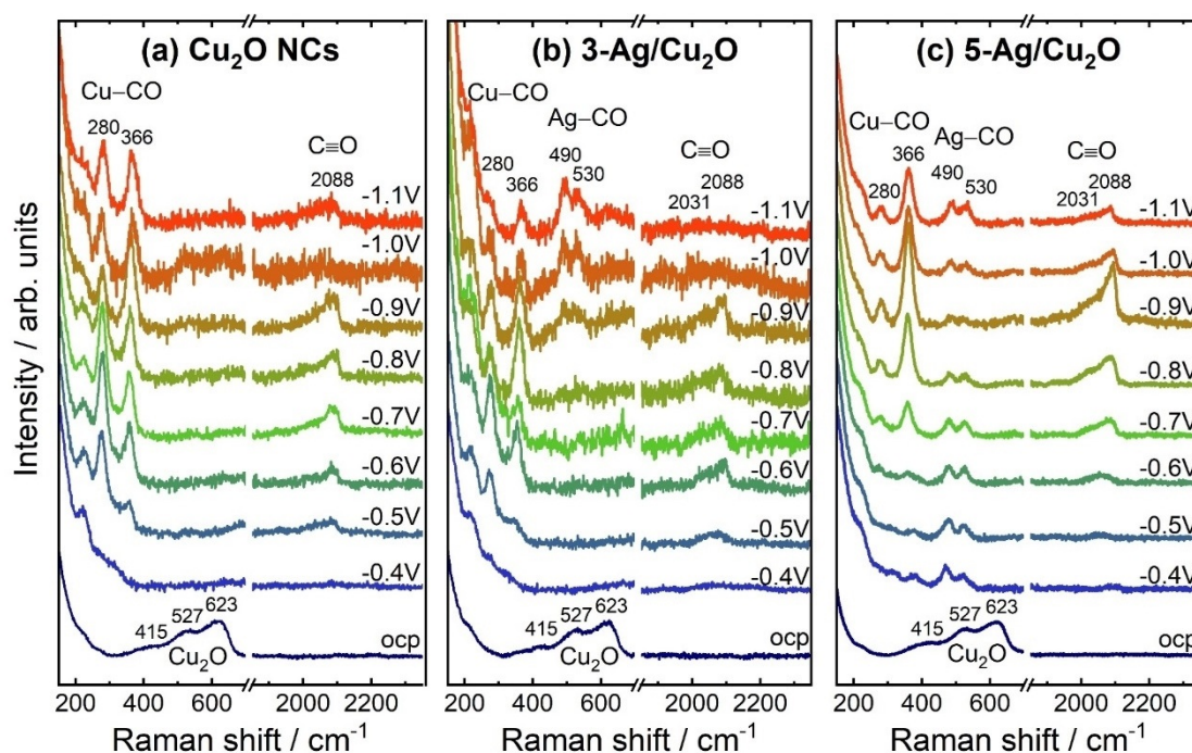
Figure 7. Operando surface-enhanced Raman spectra of a) Cu 2 O NCs, b) 3-Ag/Cu 2 O, and c) 5-Ag/Cu 2 O at open circuit potential (ocp) and under different applied potentials in CO 2 -saturated 0.1 M KHCO 3 . All potentials are given with reference to RHE.
