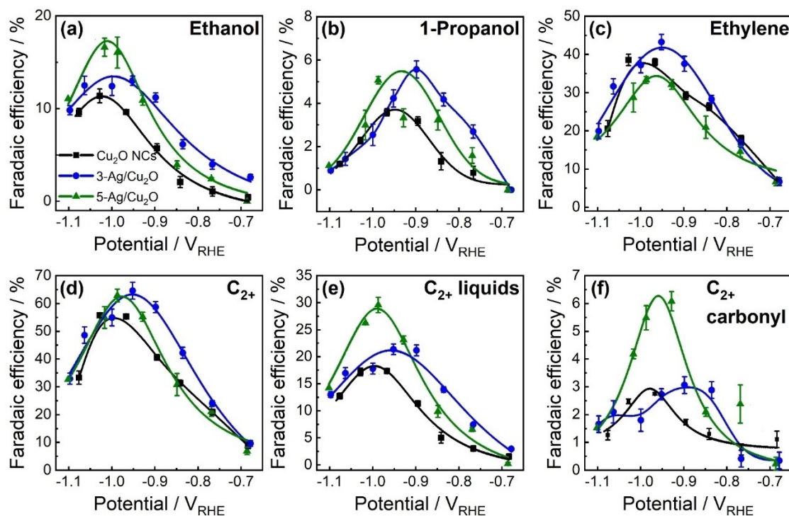
Figure 4. Potential-dependent Faradaic efficiencies of a) ethanol, b) 1-propanol, c) ethylene, d) C 2 + C 3 products (C 2+ ), e) C 2+ liquid products, and f) C 2+ carbonyl products of Cu 2 O NCs (black), 3-Ag/Cu 2 O (blue), and 5-Ag/Cu 2 O (green) after 2 h of electrolysis in CO 2 -saturated 0.1 M KHCO 3 . Solid lines are a guide for the eye.
