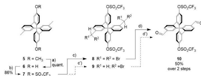
Scheme 3. Synthesis of building-block 8 . a) \text{BBr}_3 , \text{CH}_2\text{Cl}_2 , -78^\circ\text{C} to RT, overnight; b) \text{Tf}_2\text{O} , pyridine, \text{CH}_2\text{Cl}_2 , RT, 1.5 h; c) \text{NBS} , \text{BPO} (cat.), \text{CCl}_4 , reflux, 4–5 h; d) DMSO, 100^\circ\text{C} , overnight; c') reaction with 2 equiv. \text{NBS} ; d') hydrolysis, then oxidation.
